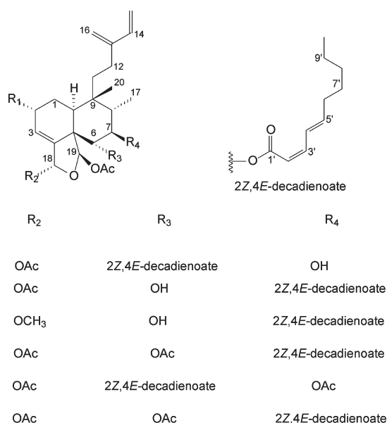
Figure 1. Structure of the clerodane diterpenes from Casearia rupestris .
